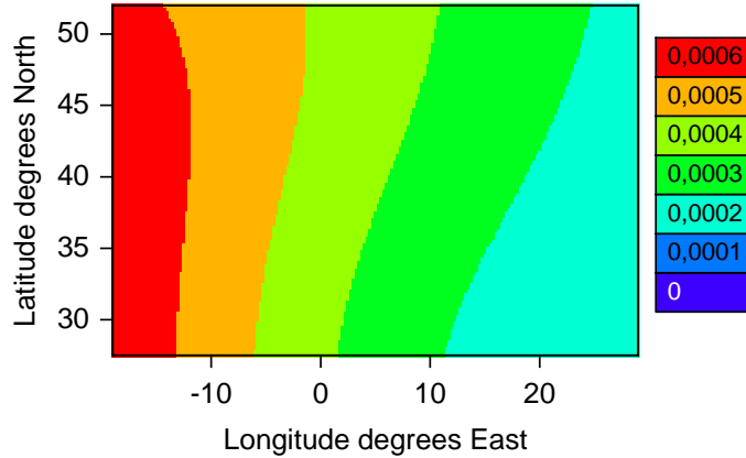
Figure 3.4.: Maritime aerosol optical depth in GRAALS.
