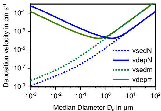
Figure 6.22.: Deposition (solid) and sedimentation (dashed) velocities for r_a=50 \text{ s m}^{-1} of number (blue) and mass (green) densities for distributions with \sigma_g=1.9 .
