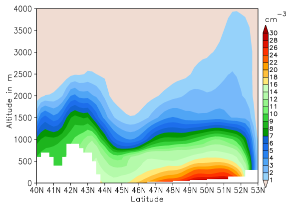
(b) Number density.
