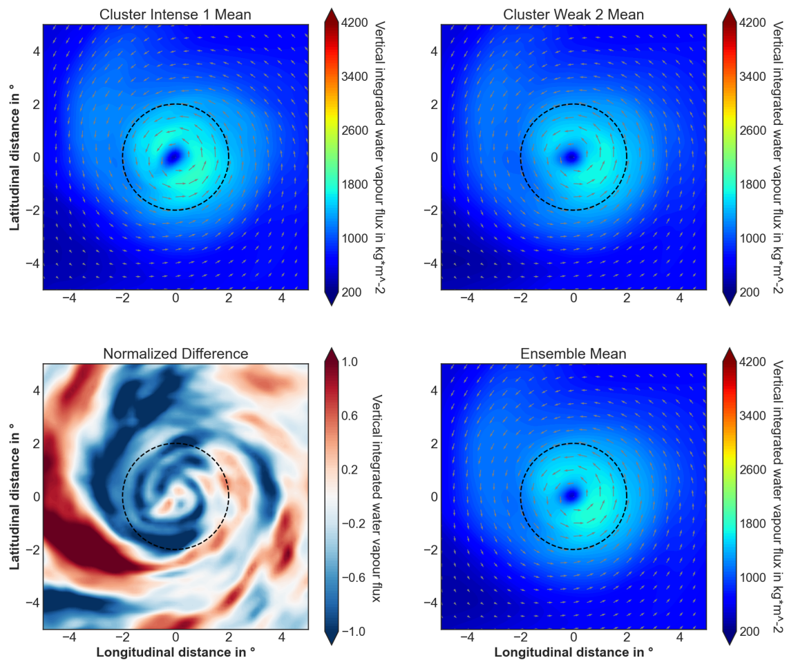
Figure 5.26: Storm-relative composites of mean vertical integrated water vapor flux after 24h forecast time for I1 (top-left), W2 (top-right), and all members (bottom-right), showing a storm after 120h. A calculated normalized difference is shown at the bottom-left. The wind field is indicated by black arrows at a pressure level of 925hPa. The black circle demonstrates the inner core of the cyclone.
