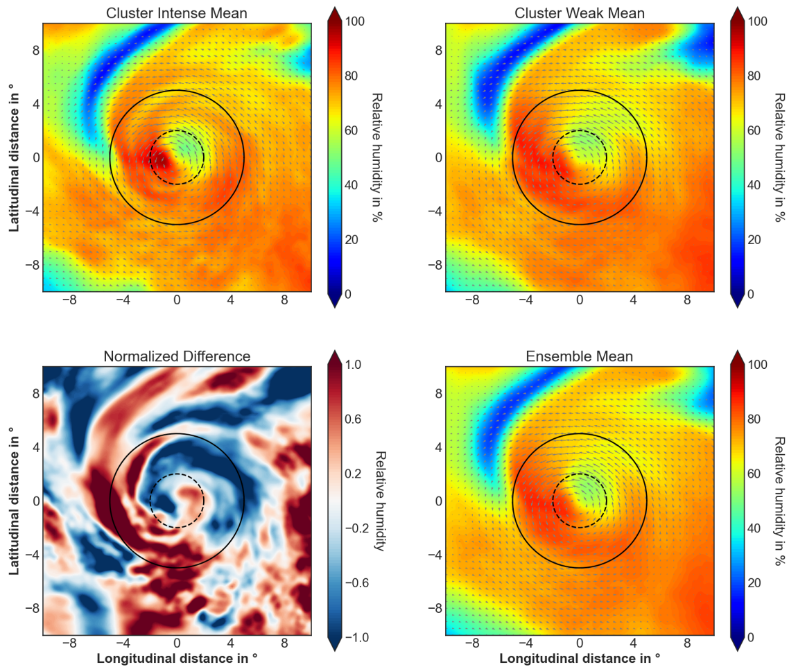
Figure 6.4: Storm-relative composites of mean relative humidity after 36 h forecast time at a pressure level of 700 hPa for I (top-left), W (top-right), and ensemble mean (bottom-right). A calculated normalized difference is shown at the bottom left. The wind field is indicated by black arrows at the corresponding pressure level. The black circle demonstrates the inner core of the cyclone.
