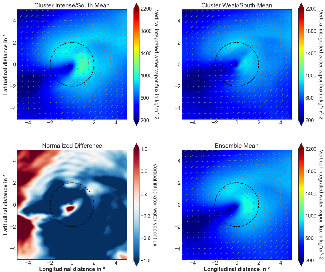
Figure 5.16: Storm-relative composites of mean VIWVF after 12 h forecast time for cluster IS (top-left), WS (top-right), and all members (bottom-right), showing a storm after 120 h. A calculated normalized difference is shown on the bottom-left. The wind field is indicated through black arrows at a pressure level of 925 hPa. The black dashed circle demonstrates the inner core of the cyclone. The area between the black dashed and solid lines represents the outer bands of the TC.
