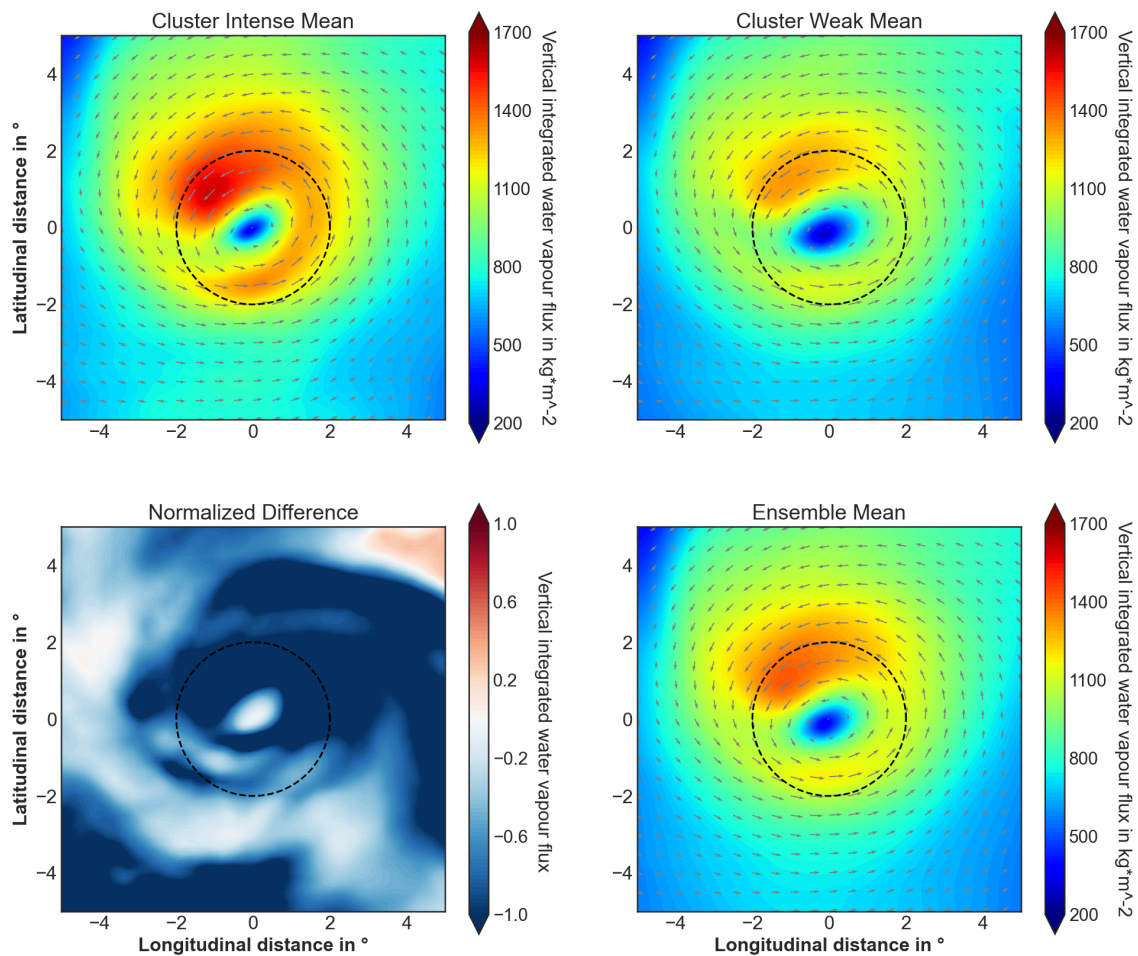
Figure 6.8: Storm-relative composites of mean VIWVF after 24 h forecast time for I (top-left), W (top-right), and ensemble mean (bottom-right). A calculated normalized difference is shown at the bottom left. The wind field is indicated by black arrows at a pressure level of 925 hPa. The black circle demonstrates the inner core of the cyclone.
