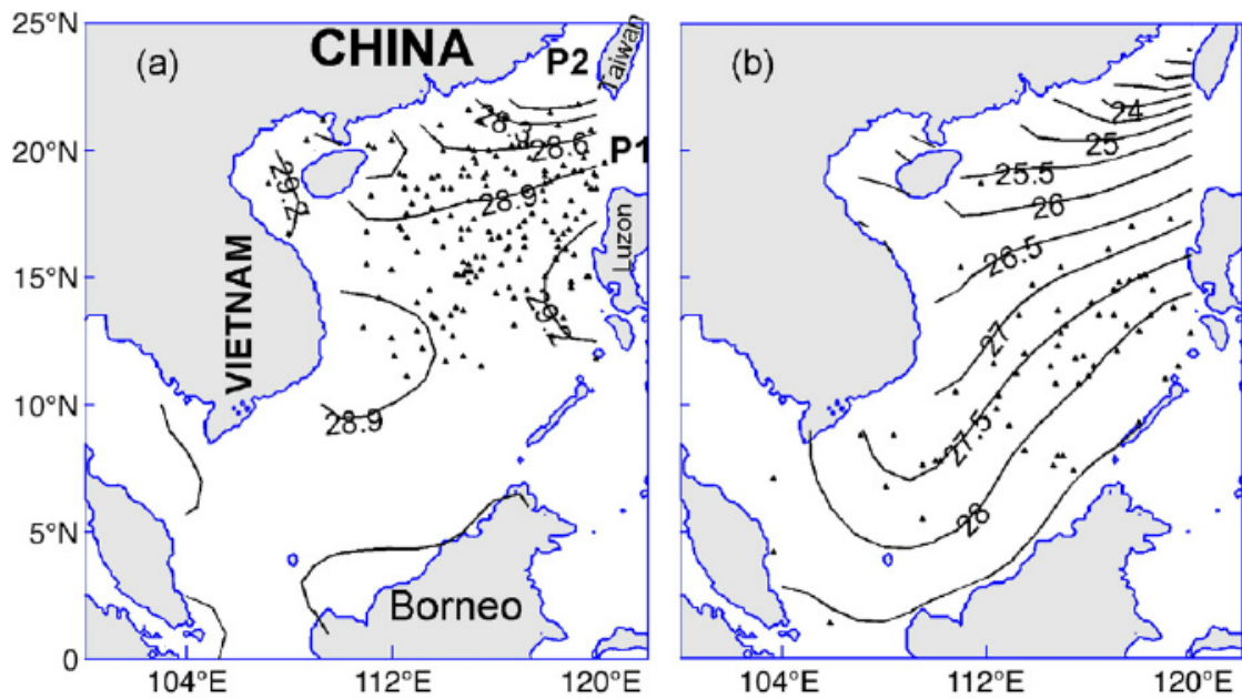
Figure 2.5: Mean climatologic sea surface temperature over the SCS between 1948 and 2003 for southwest monsoon (left) and northeasterly monsoon (right). Additionally, the genesis initial points of all storms are indicated (Wang et al., 2007)
