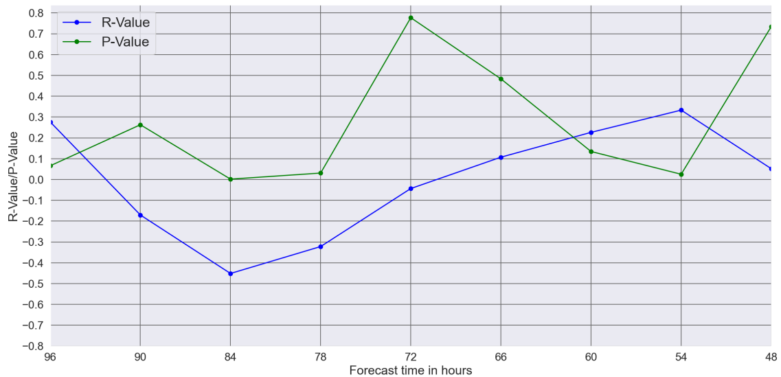
Figure 4.9: Correlation coefficient (r-value) and statistical significance (p-value) between the meridional wind at the 925hPa pressure level for the time steps between 48 and 96h and the minimum pressure at 120h for TC Atsani.
