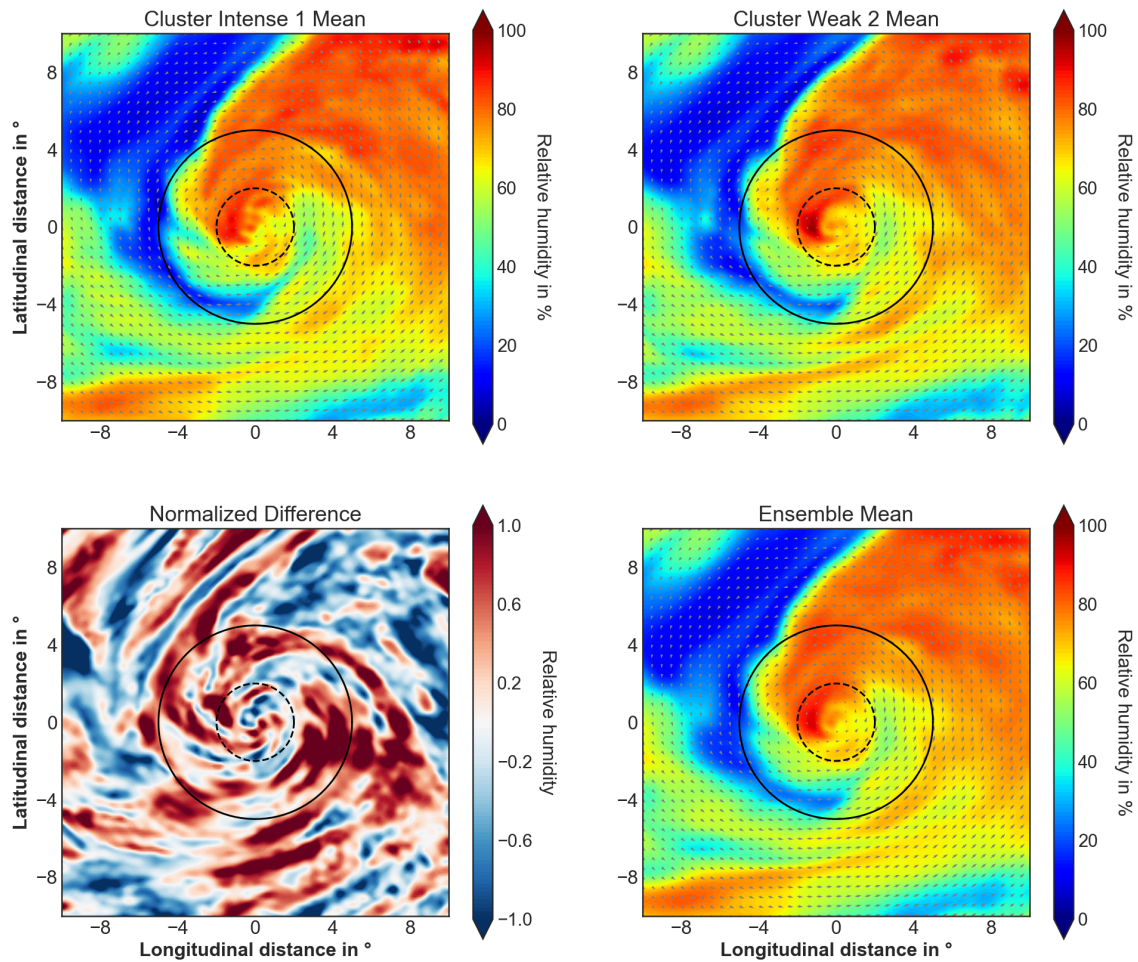
Figure 5.22: Storm-relative composites of mean relative humidity after 12 h forecast time at a pressure level of 700 hPa for I1 (top-left), W2 (top-right), and ensemble mean (bottom-right). The calculated normalized difference is shown bottom-left. The wind field is indicated by black arrows at the corresponding pressure level. The black dashed circle demonstrates the inner core of the cyclone. The area between the black dashed and solid line represents the outer bands of the TC.
