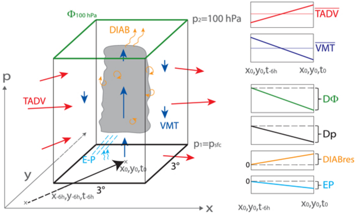
Figure 4.10: Schematic illustration of the PTE computation. The bold arrow in the x - y plane illustrates the motion of the center of a PTE during a period of 6 h. The surface pressure tendency equation is evaluated for the 3^\circ \times 3^\circ latitude-longitude box extending from the surface to the upper boundary centered on the storm's position at the initial time. The terms of (Eq.4.5), TADV (horizontal advection; red arrows), and VMT (vertical advection; dark blue vectors) are calculated by integrating over the box volume and then averaging over the period as schematically demonstrated in the two graphs in the top-right corner. The computation of the terms D\phi , Dp , and DIAB (diabatic processes curled orange vectors), and EP (evaporation minus precipitation; curled blue vectors and dashed blue lines) is indicated in the lower four graphs on the right-hand side. While D\phi and Dp are simple differences between instantaneous values over six hours, EP is the difference between two parameters accumulated between the period. DIAB_{RES} is the residuum of (Fink et al., 2012, Eq.4.5)
