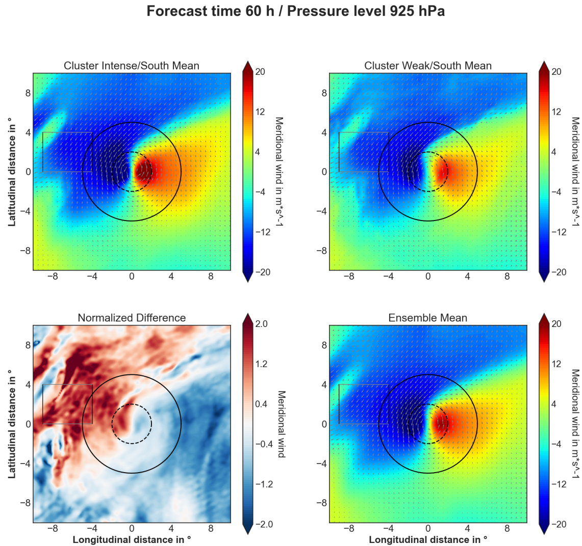
Figure 4.8: Meridional wind and stream field at 925 hPa for TC Atsani at 60h forecast time. The black dashed line indicates the center and the inner storm area. The area between the black and black dashed line demonstrates the outer bands of the storm. The gray solid line shows the area for mean meridional wind computation for cluster intense (top-left), cluster weak (top-right), normalized difference (bottom-left), and the ensemble mean (bottom-right).
