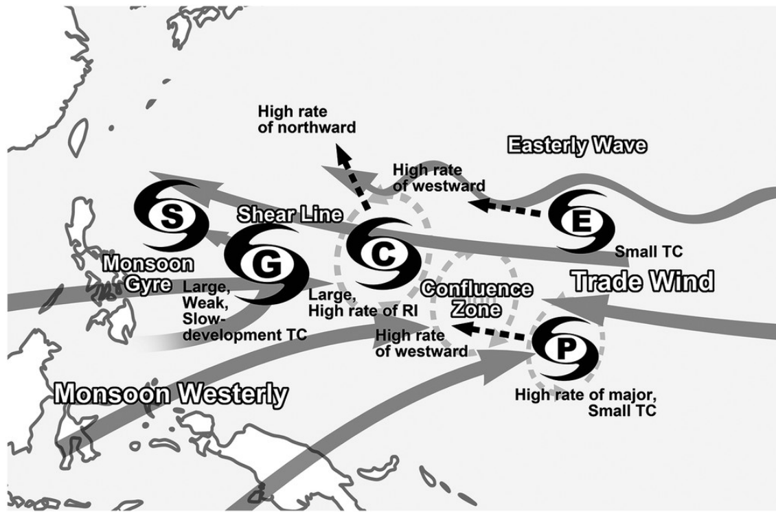
Figure 2.4: Schematic image of the five different flow patterns leading to TCG. TCG location is indicated and the westerly and easterly winds are illustrated by arrows (Fudeyasu and Yoshida, 2018).
