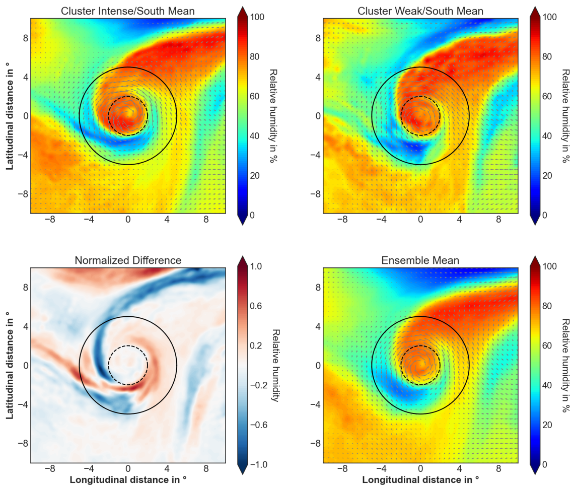
Figure 5.4: Same as Fig.5.3 but after 72 h forecast time.
